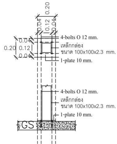
DETAIL CX
